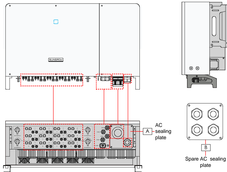
Fig.2. Wiring Terminals (Take SG250HX as an example)
