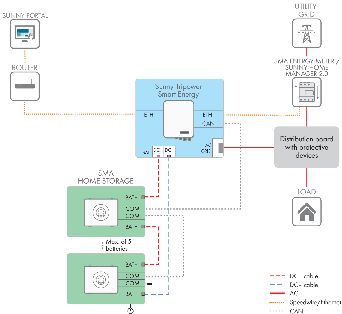
Figure 16: SMA Home Storage with 1 hybrid inverter (example)
