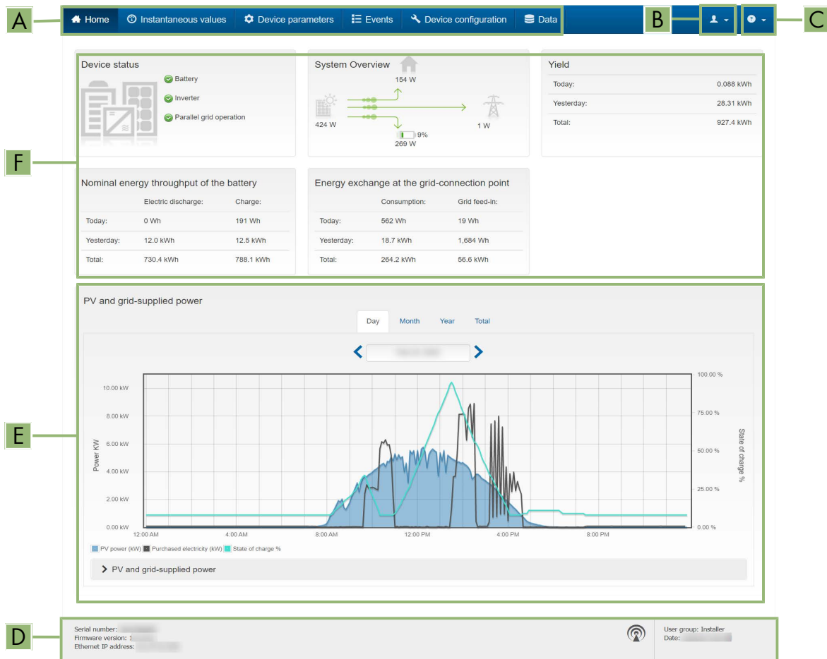
Figure 18: Design of the user interface's home page (example)
