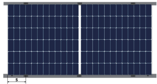
Installation of frameless module with fixtures on long sides (clamp length = 150mm)
