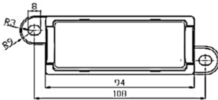
Fuse holder for MEGA-fuse
